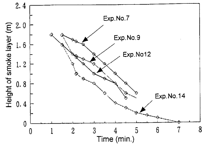
Fig.8 Height of smoke layer from the floor in lapse of time.
