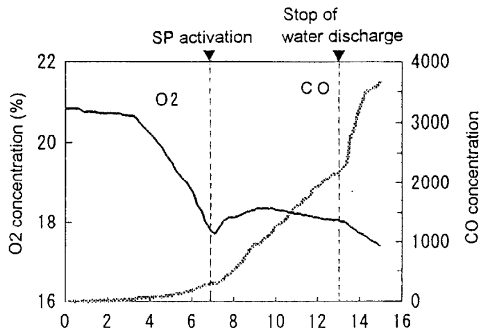
Fig.9 O 2 and CO concentrations in lapse of time for the experiment No.8.
