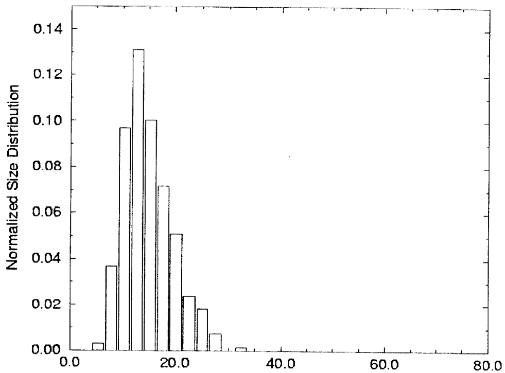
Figure 2b. The normalized water droplet distribution at the nozzle exit for strain rate of 285 \text{ s}^{-1} .
