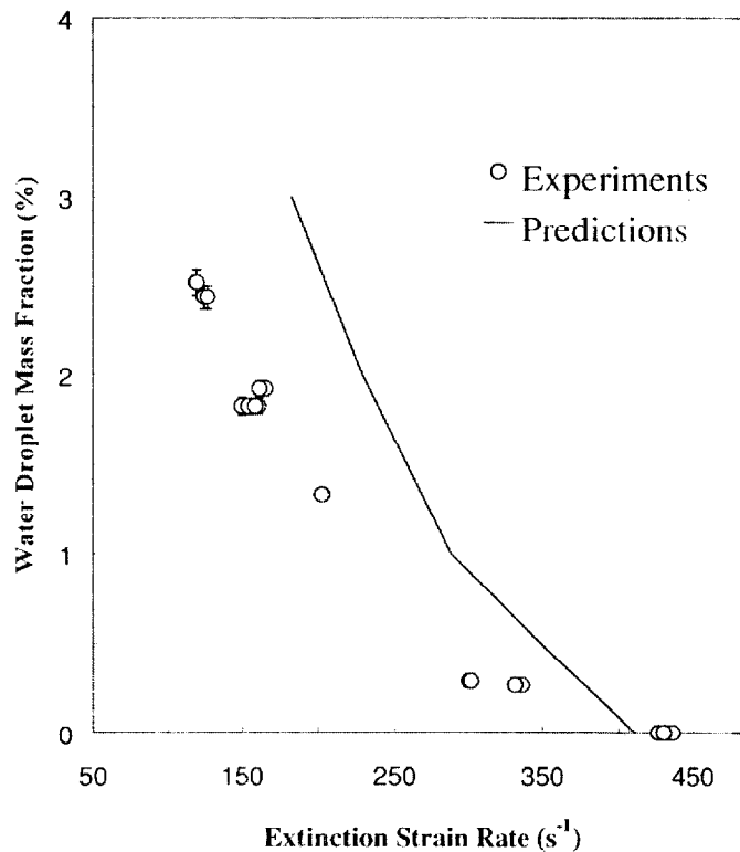
Figure 3. Condensed phase water droplet mass fraction as a function extinction strain rate.
