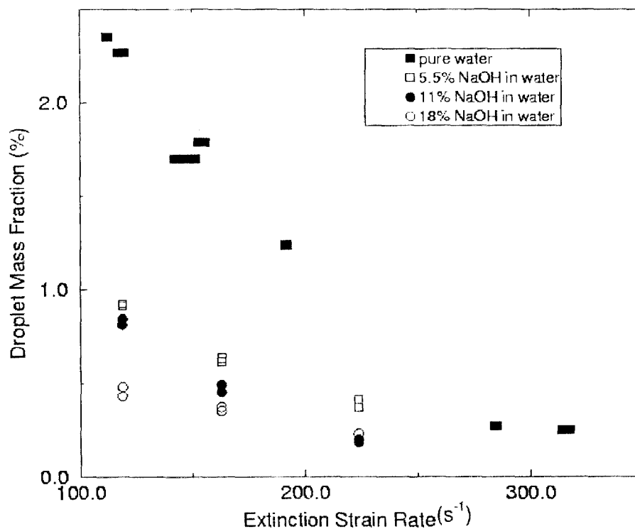
Figure 4. Comparison of the condensed phase droplet mass fraction as a function of extinction strain rate, for different mass loading of NaOH in water.
