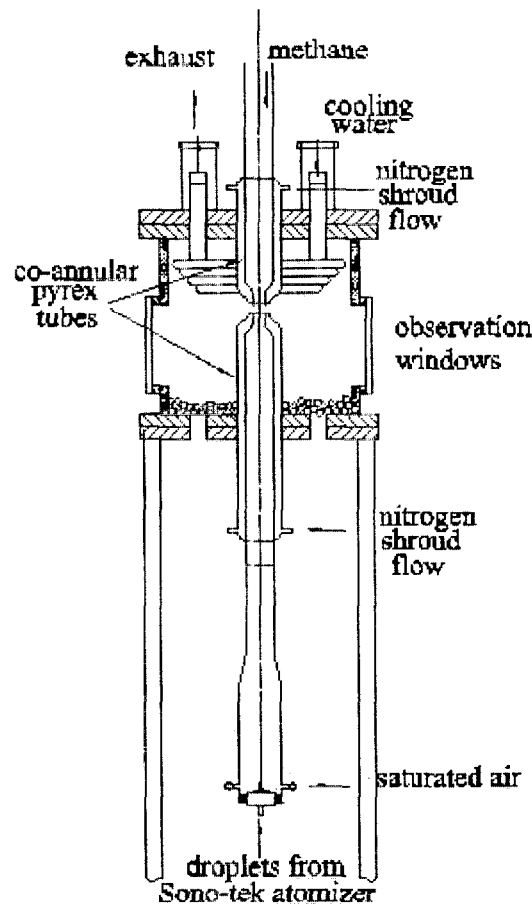
Figure 1. Counterflow burner configuration with the Sono-Tek water droplet atomizer.
