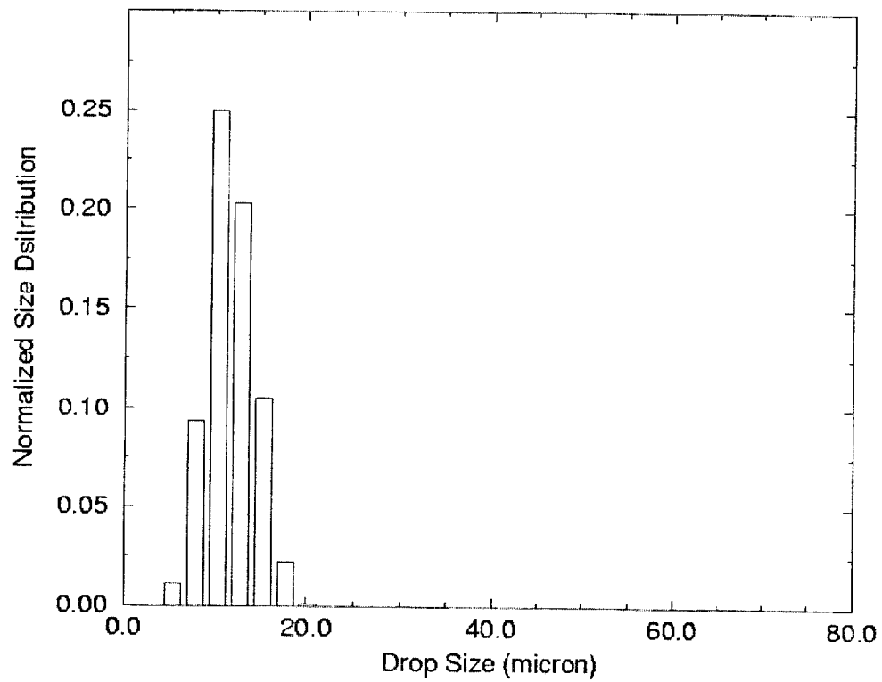
Figure 2a. The normalized water droplet distribution at the nozzle exit for strain rate of 160 \text{ s}^{-1} .
